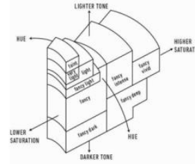
Illustration of GIA fancy color grade interrelationships
